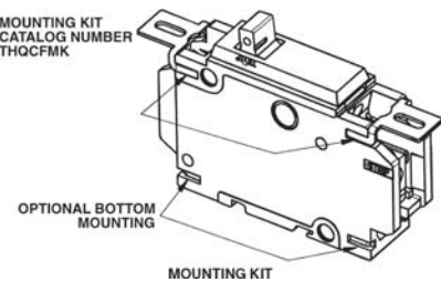
Mounting Kit THQCFMK
